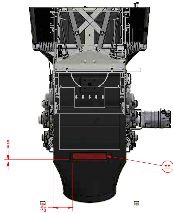
VIEW AG-AG
