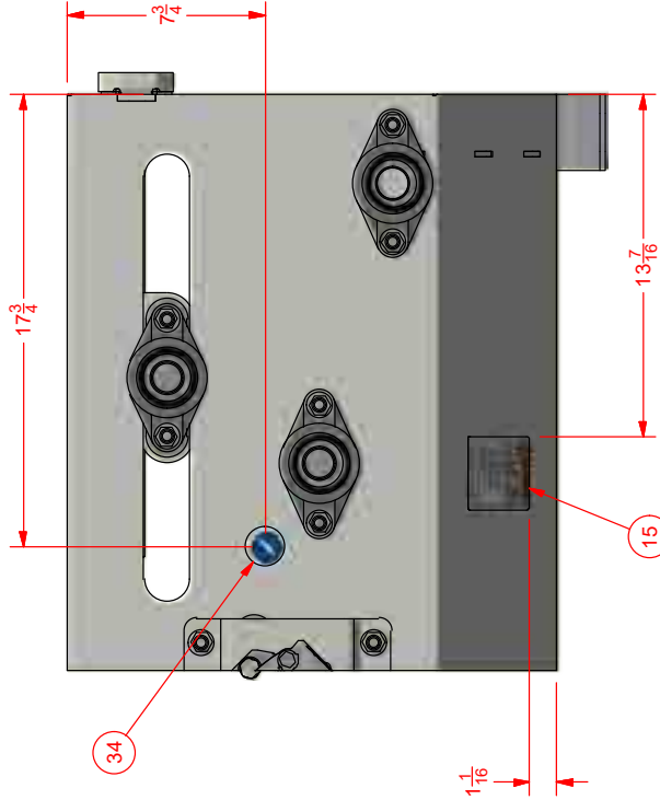
VIEW B-B
