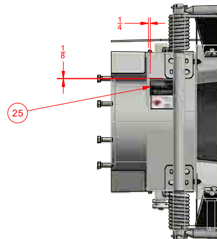
VIEW AE-AE
