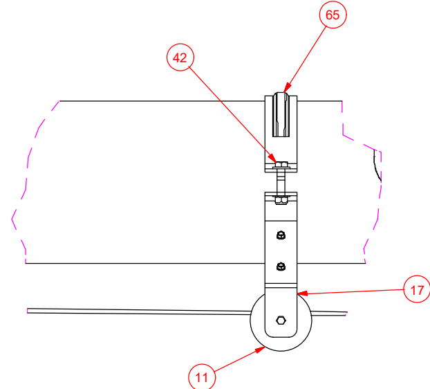
DETAIL D
